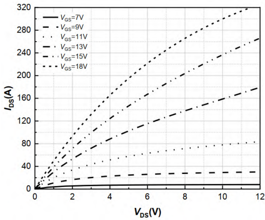
Fig 3 Typical Output Characteristics ( T_J = 25^\circ\text{C} )
