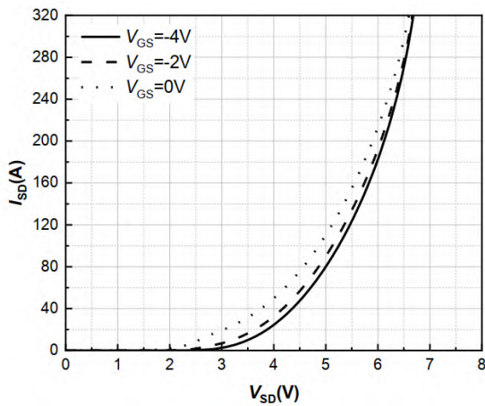
Fig 11 Body-Diode Characteristics ( T_J = 25^\circ\text{C} )
