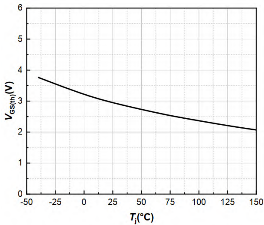
Fig 5 V_{GS(th)} vs. Junction Temperature
