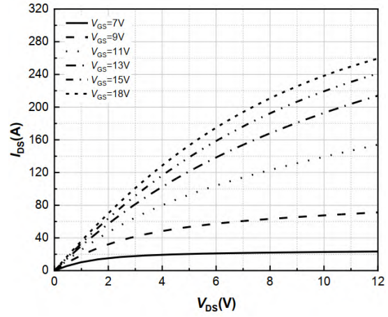
Fig 4 Typical Output Characteristics ( T_J = 150^\circ\text{C} )
