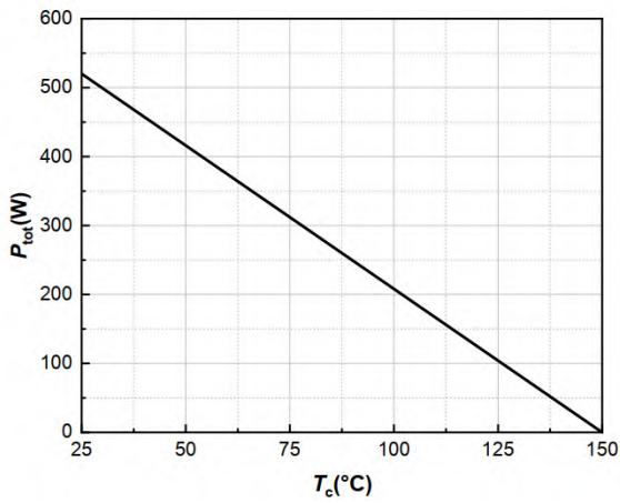
Fig 1 Power Dissipation
