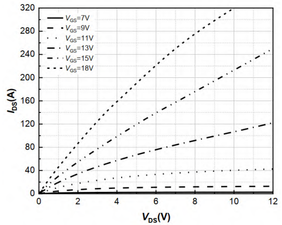
Fig 2 Typical Output Characteristics ( T_J = -40^\circ\text{C} )
