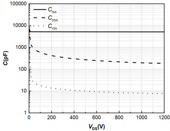
Fig 13 Capacitance Characteristics
