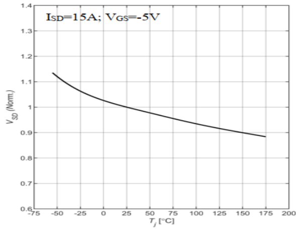
Fig 9 Normalized Diode Forward Voltage vs. Junction Temperature
