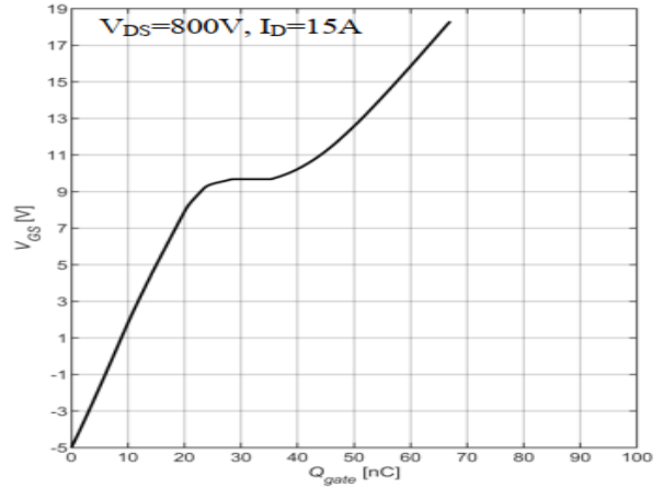
Fig 14 Gate-Charge Characteristics
