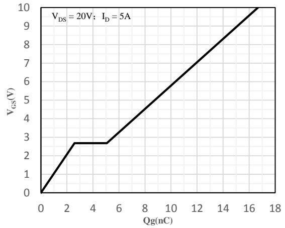
Fig 10 Gate-Charge Characteristics
