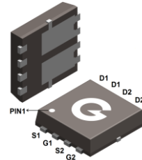
PDFN3×3-8LC
