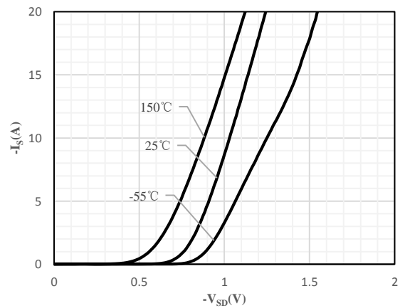
Fig 6 Body-Diode Characteristics
