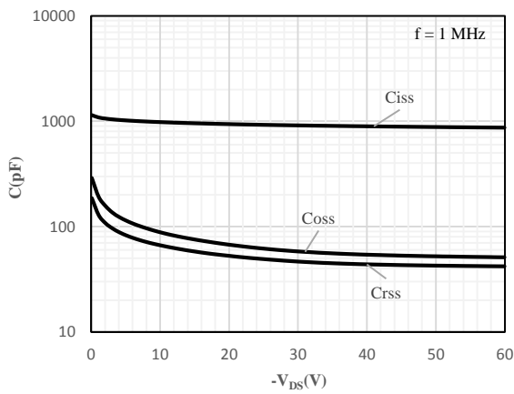
Fig 9 Capacitance Characteristics
