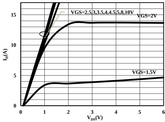
Fig 3 Output Characteristics
