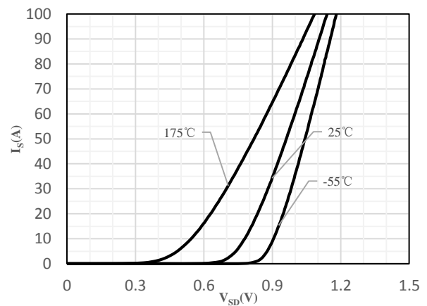
Fig 6 Body-Diode Characteristics
