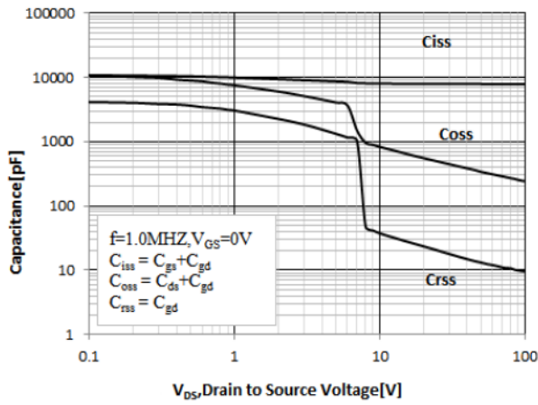
Fig 9 Capacitance Characteristics
