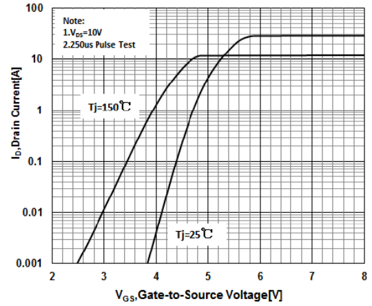
Fig 8 Transfer Characteristics
