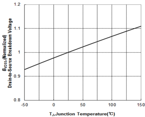
Fig 11 Normalized Breakdown Voltage vs. Junction Temperature
