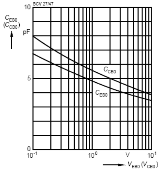
Emitter-base capacitance C_{EB} = f(V_{EB0})
